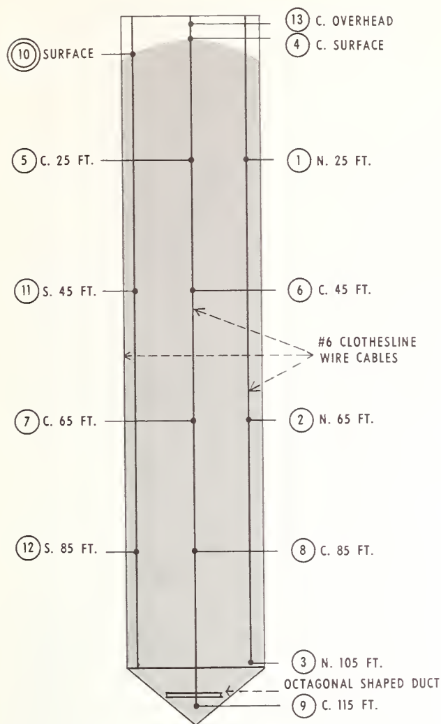
FIGURE 2.—Location of the aeration duct and the gas sampling points throughout the column of grain.
